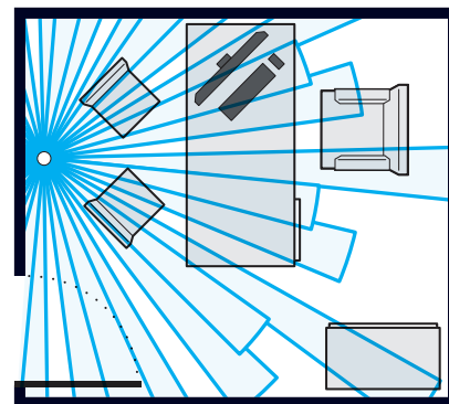
Diagram 1 - Recommended Sensor Placement in a Private Office
